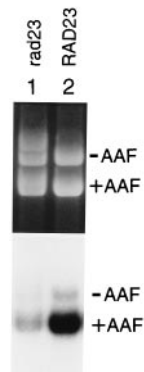
FIG. 2. NER in rad23 deletion mutant extract. In vitro NER was performed in 300 \mu g of rad23 deletion mutant extract (lane 1) or its isogenic wild-type extract (lane 2) at 26°C for 2 h. +AAF, pUC18 DNA containing AAF adducts; -AAF, undamaged pGEM-3Zf(+) DNA. Top, ethidium bromide-stained gel; bottom, autoradiogram.
