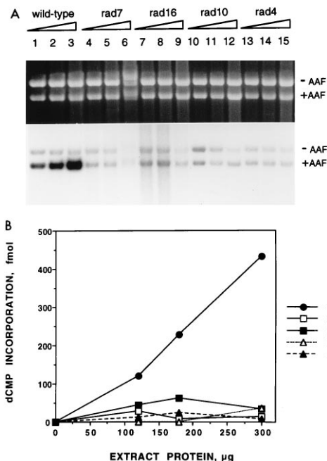
FIG. 1. NER in rad7 and rad16 deletion mutant extracts. (A) In vitro NER was performed in various yeast cell extracts as indicated with extract concentrations at 120 \mu g (lanes 1, 4, 7, 10, and 13), 180 \mu g (lanes 2, 5, 8, 11, and 14), and 300 \mu g (lanes 3, 6, 9, 12, and 15). Repair reactions were at 26°C for 2 h, and the repair products were processed as described in Materials and Methods. +AAF, pUC18 DNA containing AAF adducts; -AAF, undamaged pGEM-3Zf(+) DNA. The top panel shows the ethidium bromide-stained gel, and the bottom panel is an autoradiogram showing DNA synthesis. (B) Damage-specific DNA repair synthesis in A was quantitated by scintillation counting of the DNA bands excised from the gel. WT, wild type.
