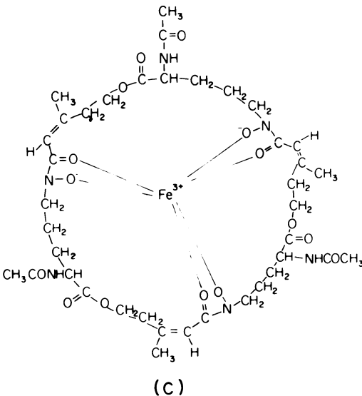
FIG. 1. Structures of A. nidulans and P. chrysogenum siderophores. (a) Ferrichrome, R = H; ferricrocin, R = CH 2 OH. (b) Coprogen. (c) N,N',N''-Triacetylfusigen.
