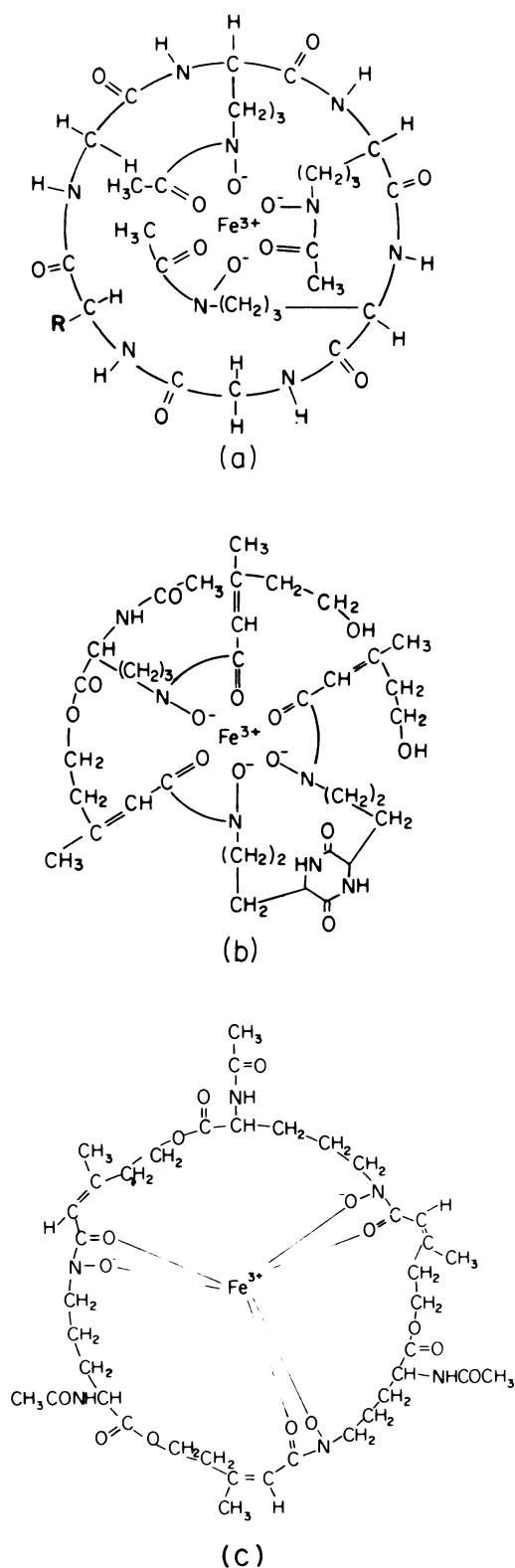
FIG. 1. Structures of A. nidulans and P. chrysogenum siderophores. (a) Ferrichrome, R = H; ferricrocin, R = CH 2 OH. (b) Coprogen. (c) N,N',N''-Triacetylfusigen.
