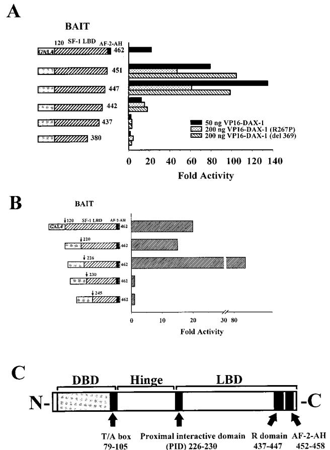
FIG. 2. Interaction between SF-1 and DAX-1 requires two domains within SF-1. CV-1 cells were cotransfected with fusions of GAL4 DBD and SF-1 carboxy terminus (20 ng), fusions of VP16 and DAX-1 (wild type [amino acids 1 to 472]), DAX-1 (R267P), or DAX-1 (del 369) (50 or 200 ng), and 250 ng of GAL4 reporter. (A) Fusions of GAL4 DBD with SF-1 amino acids 120 to 462, 120 to 451, 120 to 447, 120 to 442, 120 to 437, or 120 to 380 were tested with a two-hybrid assay against all three forms of VP16-DAX-1. Only activity from VP16-DAX-1 (wild type) is shown for GAL4-SF-1 (amino acids 120 to 462). (B) Fusions of GAL4 DBD with SF-1 amino acids 120 to 462, 220 to 462, 226 to 462, 230 to 462 or 245 to 462 were tested in a two-hybrid assay against VP16-DAX-1 (wild type). Luciferase activities were measured and standardized as described in Materials and Methods. Fold activities were calculated by determining the degree of enhancement by VP16-DAX-1 of the activity of each GAL4-SF-1 construct compared to the degree of enhancement observed with GAL4 DBD (see Materials and Methods). (C) Schematic diagram of SF-1, demonstrating the DBD, T/A box, PID, R domain, and AF-2-AH. See text for details.
