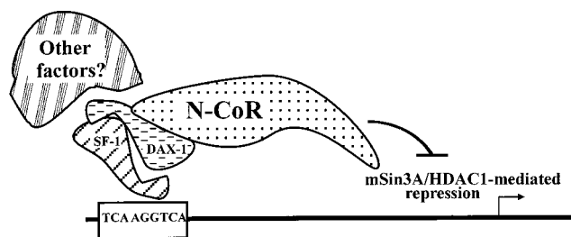
FIG. 7. Schematic model of mechanism of DAX-1 repression of SF-1. SF-1, bound to its response element on DNA, recruits DAX-1, requiring the PID and the R domain within the carboxy terminus of SF-1. To interact with SF-1, DAX-1 employs its structurally degenerate DBD (30). DAX-1 in turn recruits N-CoR to DNA, requiring at least two conserved regions within DAX-1 LBD, either of which is mutated or eliminated in different AHC kindreds. Other molecules may stabilize or modify the interaction among the three proteins, depending on the cell or promoter context.
