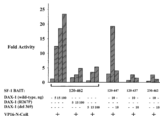
FIG. 5. DAX-1 potentiates two-hybrid interaction between SF-1 and N-CoR. CV-1 cells were cotransfected with GAL4 DBD fusions of the SF-1 carboxy terminus (amino acids 120 to 462, 120 to 447, 120 to 437, or 230 to 462) (20 ng), VP16-N-CoR (20 ng [Fig. 5]); increasing amounts of wild-type, mutant R267P, or del 369 DAX-1 (0, 5, 10, 15, or 100 ng); and GAL4 reporter (250 ng). Luciferase activities were measured and standardized as described in Materials and Methods. Fold activities were calculated by determining the degree of enhancement by VP16-N-CoR of the activity of each GAL4-SF-1 construct in the presence or absence of DAX-1 constructs compared to the degree of enhancement observed with GAL4 DBD (see Materials and Methods).
