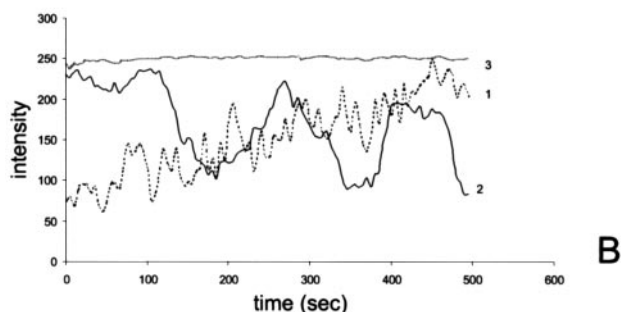
FIG. 3. (A) Figure corresponding to time-lapse series 1 (available online); individual FMRP-GFP labeled granules were observed by time-lapse microscopy. The time-lapse series shows the movement of green fluorescent granules in PC12/FMR7 cells after DOX induction (2 h) in a time-lapse study of frames every 5 s for 500 s. Note the movement of fluorescent granules between the swelling along the neurite (square 2) and the growth cone (rectangle 1). (B) Quantification of the emission intensities over time (500 s). The overall emission intensity in the cell body (square 3) remains the same over time, whereas the emission intensity within the swelling (square 2) follows a cycle every 3 min. The emission profile of the growth cone shows a gradual increase of intensity during the recorded time (rectangle 1).
