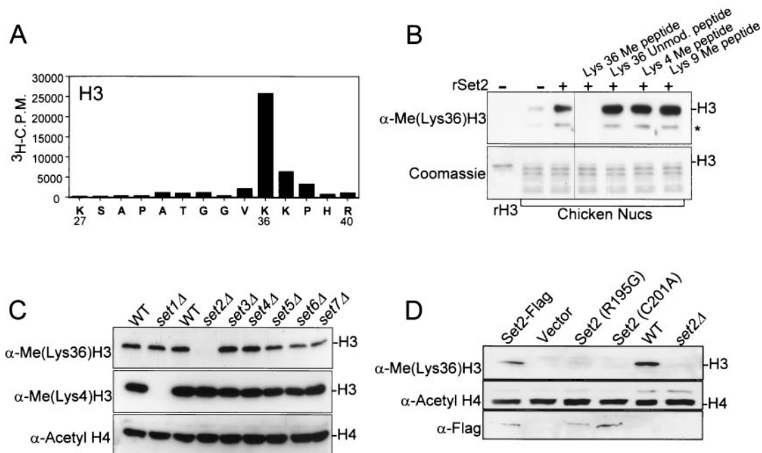
FIG. 5. Methylation of H3 at lysine 36 is mediated by Set2. (A) RP-HPLC-purified H3 isolated from Set2 reactions involving ^3\text{H} -AdoMet and chicken nucleosomes was digested with endoproteinase Glu-C, and the resulting peptide fragments were separated by RP-HPLC. A labeled H3 fragment, determined to be amino acids 1 to 50 by mass spectrometry (data not shown), was further digested with the endoproteinase Arg-C followed by RP-HPLC fractionation. From this digestion, a ^3\text{H} -methylated peptide fragment identified as being amino acids 27 to 38 in H3 by mass spectrometry (data not shown) was subjected to N-terminal automated sequencing, and ^3\text{H} radioactivity eluted from each cycle was counted. Amino acids identified at each cycle of microsequencing are listed; numbers correspond to the known positions of H3 residues. (B) Recombinant H3 or chicken nucleosomes reacted in the presence or absence of purified recombinant Set2 along with AdoMet were immunoblotted with the \alpha -Me(Lys36)H3 antiserum (upper panel). Identical reactions were performed and used in peptide competition assays in which the \alpha -Me(Lys36)H3 antiserum was incubated for 2 h at 25°C with the various peptides shown (peptides were at 10 \mu\text{g}/\text{ml} ). Parallel reactions were performed and examined by Coomassie staining to monitor loading (lower panel). Asterisk indicates the partial H3 breakdown product observed. (C) Set2 mediates H3 Lys36 methylation in vivo. Whole-cell extracts from wild-type S. cerevisiae strains or strains with a deletion of the SET domain were probed with either the \alpha -Me(Lys36)H3 antiserum, the \alpha -Me(Lys4)H3 antiserum, or the \alpha -acetyl-H4 antiserum (used for a loading control). Details of the S. cerevisiae strains used are as follows (from left to right as shown in the panel): WT (MBY1198), set1 \Delta (YHR119w), WT (BY4742), set2 \Delta (YJL168c), set3 \Delta (YKR029c), set4 \Delta (YJL105w), set5 \Delta (YHR207c), set6 \Delta (YPL165c), and set7 \Delta (YDR257c). MBY1198 and BY4742 are the isogenic wild-type strains for the set1 \Delta and set2 \Delta to set7 \Delta strains, respectively. (D) The SET domain of Set2 is essential for mediating H3 Lys36 methylation in vivo. Whole-cell extracts from wild-type, set2 \Delta , and set2 \Delta strains with either the vector control plasmid (Vector), wild-type Set2 expression plasmid (Set2-Flag), or either of the SET domain mutants [Set2 (R195G) and Set2 (201A)] were probed with the \alpha -Me(Lys36)H3 antiserum. For a loading control, these extracts were probed with the \alpha -acetyl-H4-specific antiserum. Expression of wild-type or mutant Set2 proteins was monitored using the anti-Flag monoclonal antiserum.
