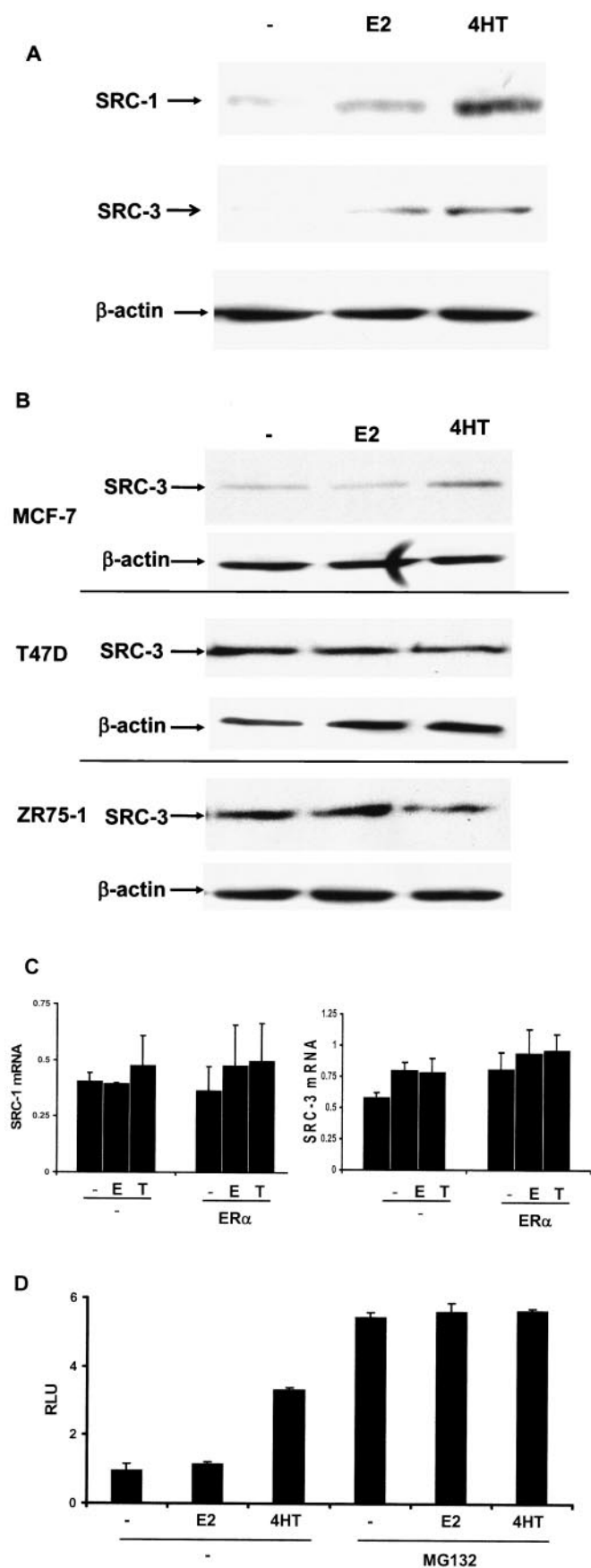
FIG. 4. 4HT can elevate endogenous SRC-1 and SRC-3 in HeLa cells transiently transfected with ER \alpha and in MCF-7 cells. (A) HeLa cells were transfected with pERE-E1b-CAT and pCR3.1 hER \alpha , incubated 24 h, and then treated with ethanol vehicle (-), E2, or 4HT for 24 h and harvested for Western analysis. (B) 4HT is able to promote elevation of endogenous SRC-3 in MCF-7 but not T-47D or ZR-75-1 ER \alpha -positive breast cancer cell lines. Untransfected MCF-7, T-47D, and ZR-75-1 cell lines were treated with ligands and harvested for Western analysis as described for panel A. (C) 4HT treatment has no effect on SRC-1 or SRC-3 mRNA levels in HeLa cells transfected with ER \alpha . HeLa cells were transfected with pERE-E1b-CAT and pCR3.1 hER \alpha and then treated for 24 h with ligands as described above. Cells were harvested for total RNA, and mRNA for SRC-1 and SRC-3 was quantitated by real-time PCR. (D) In MG132-treated HeLa cells, SRC-1A-LUC protein is not further elevated when cotreated with 4HT. HeLa cells were transfected with pERE-E1b-CAT, pCR3.1hER \alpha , or pCR3.1 SRC-1A-LUC and treated with ethanol vehicle (-), E2, or 4HT with or without MG132 for 8 h and harvested for luciferase activity.
