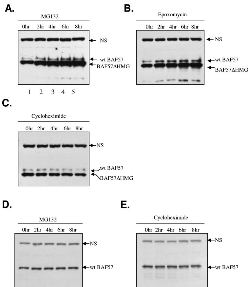
FIG. 2. Inhibition of proteasome and translation has distinct effects on the BAF57 protein level in UL3 and UL3/BAF57ΔHMG-1 cells. UL3/BAF57ΔHMG-1 cells were treated with either MG132 (A), epoxomycin (B), or cycloheximide (C) for 0, 2, 4, 6, and 8 h. Whole-cell extracts were prepared at each time point and resolved by 12% SDS-PAGE. The relative protein levels of wt BAF57 and BAF57ΔHMG in the extracts were determined by Western blotting. UL3 cells were also treated with either MG132 (D) or cycloheximide (E) for 0, 2, 4, 6, and 8 h. The relative protein level of wt BAF57 present at each time point was again determined by Western blotting. “NS” denotes a nonspecific band recognized by the BAF57 antibody and indicates equivalent loading.
